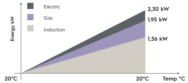
Energy required to heat 12 liters of water from 20° to 90°C
